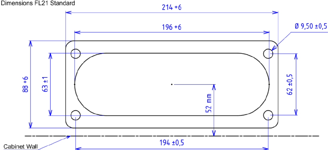
Dimensions FL21 Standard
